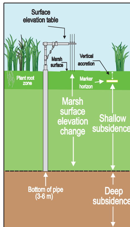
Fig. 3. Methods used to measure marsh elevation change and shallow subsidence.
